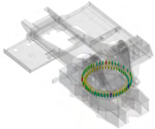
3D stress diagram for bolts
