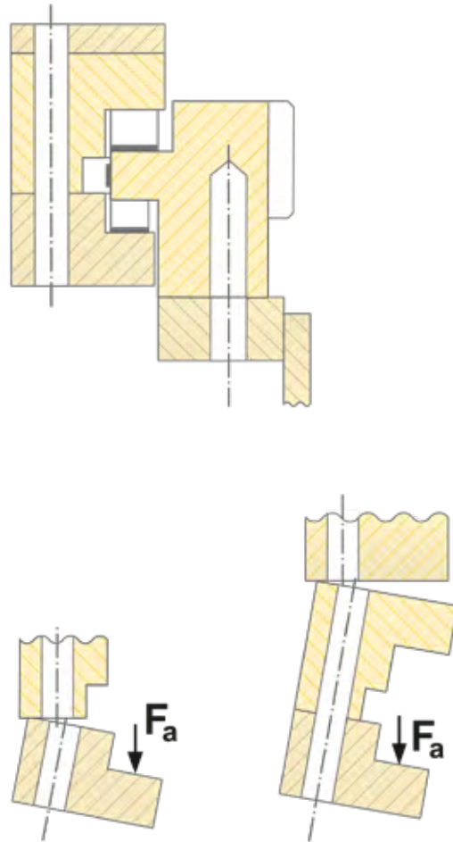
Example 2: Gaping of bearing rings i.a.w. DNV GL
