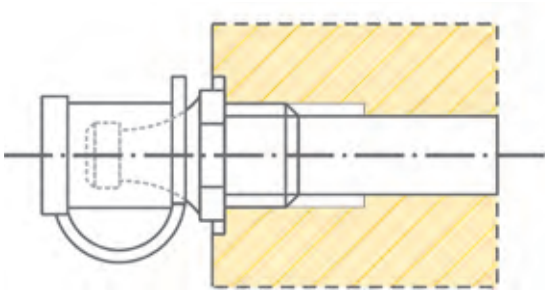
Lubrication port with threaded nipple
