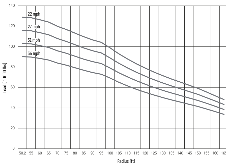
The above diagram shows an example of the selectable load curves for different wind speeds.
